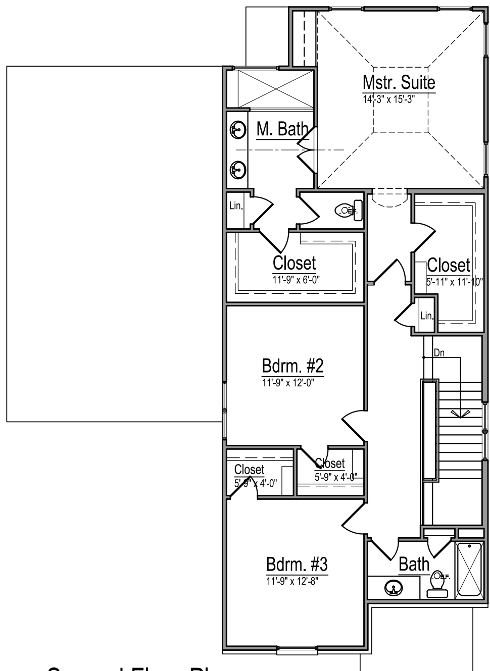
Second Floor Plan Total: 1,104 SQ. FT.
