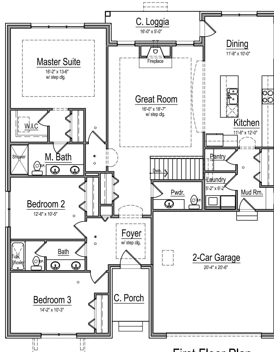
First Floor Plan 1,887 SQ. FT.
